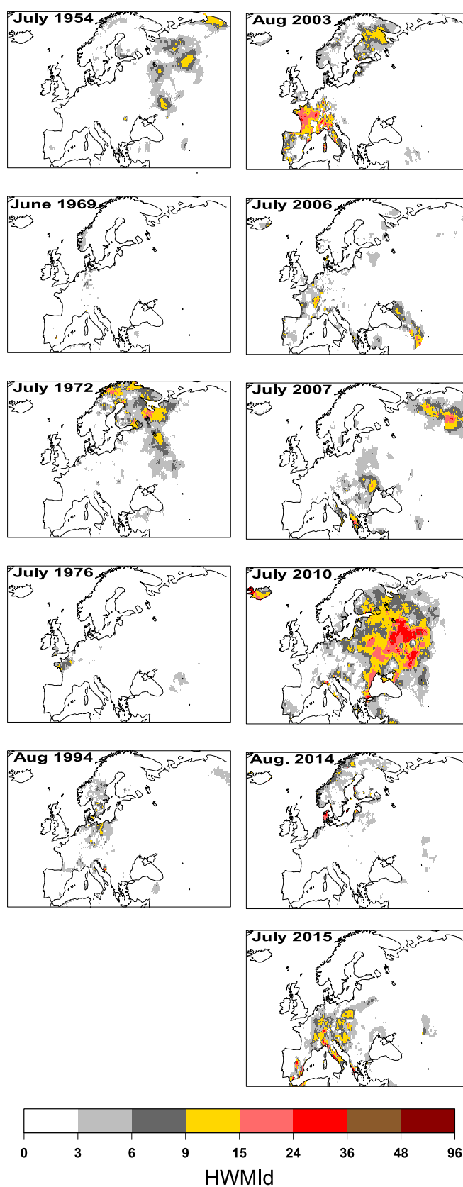
Figure A2. As figure 2 but for HWMI calculated with daily minimum temperatures.
