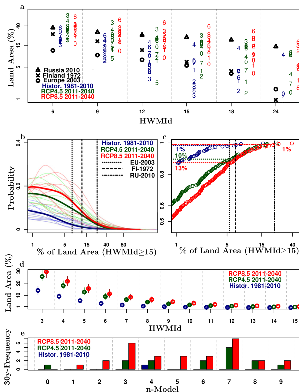
Figure 3. Empirical probability and cumulative distribution functions (EPDFs and ECDFs) of the percentage land area in heatwaves. (a) Percentage of EURO-CORDEX land area covered by HWMId maximum values greater than a given magnitude level ( \text{HWMId} \geq 6, 9, \dots, 24 ) for the 2003, 1972, and 2010 European heatwaves with E-OBS data (black) and for the strongest heatwave simulated by each individual model in the periods 1981–2010 and 2011–2040. The numbers from 0 to 9 refer to heatwaves simulated by individual models (see table A.1). Hence, as an example, at the RCP8.5 level the heatwave with the strongest magnitude and spatial extent simulated by the model 0, in 2011–2040 and under the RCP8.5 scenario, is represented by the red symbol 0. (b) PDFs of the percentage land area covered by grid points with HWMId values equal to or greater than 15. The PDFs are shown for the period 1981–2010 (blue curves) and 2011–2040 under RCP4.5 (green curves) and RCP8.5 (red curves) scenarios. The transparent coloured lines mark individual EURO-CORDEX models, comprised of 30 year values, whereas the bold colored curves represent the PDFs comprised of all 300 (30 years X 10 models) model years. Dotted and dashed lines denote the observed (E-OBS) 2003 and 2010 events, respectively. (c) As (b) but for ECDF of 300 model years. Each open circle represent the percentage of area (value on x-axis) and the corresponding probability for a single model year. The horizontal dashed and dotted lines denote the probability to have 2003 and 2010 type heatwave in 30 year period and under a specific scenario. (d) Percentage of area versus different HWMId levels. The open colored circles and the error bars represent the median and the range of the bootstrap applied at each HWMId level to the ECDF of 300 model years (see panel (c) for \text{HWMId} \geq 15 ). (e) Occurrence of a 2003-type heatwave in present and near future periods of 30 year simulated by each model according to the ranking method in section 2.8.
