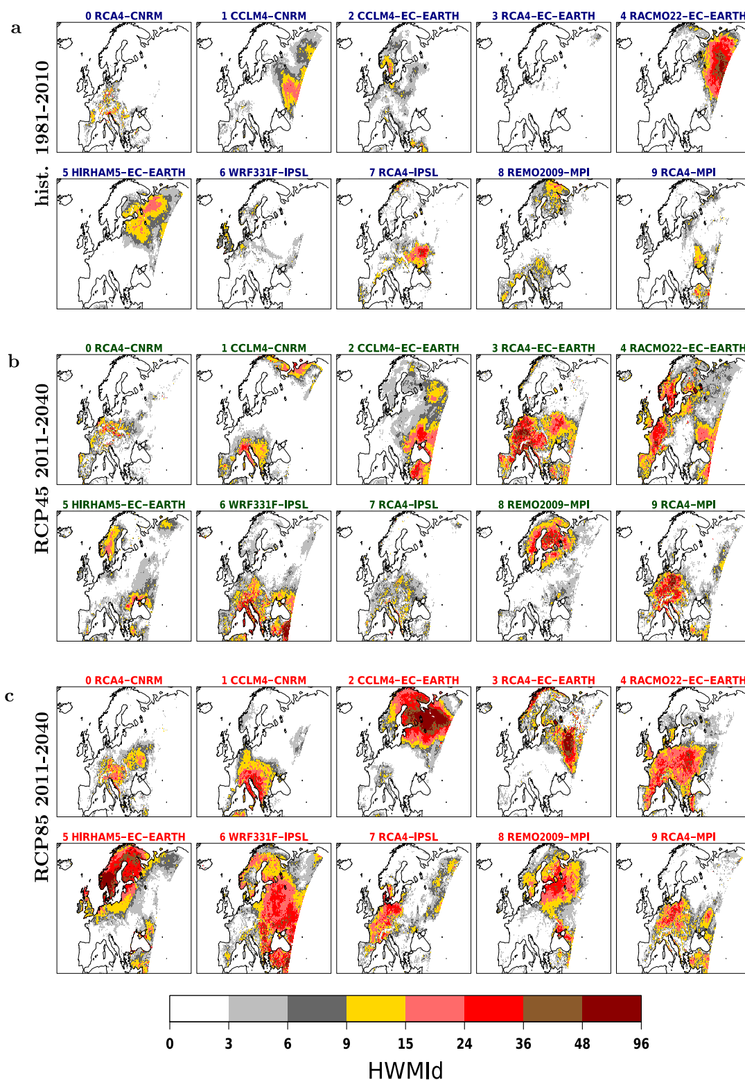
Figure A4. As figure 5 but for HWMI calculated with T_{min} in the same model year of the strongest heatwaves represented in figure 5.
