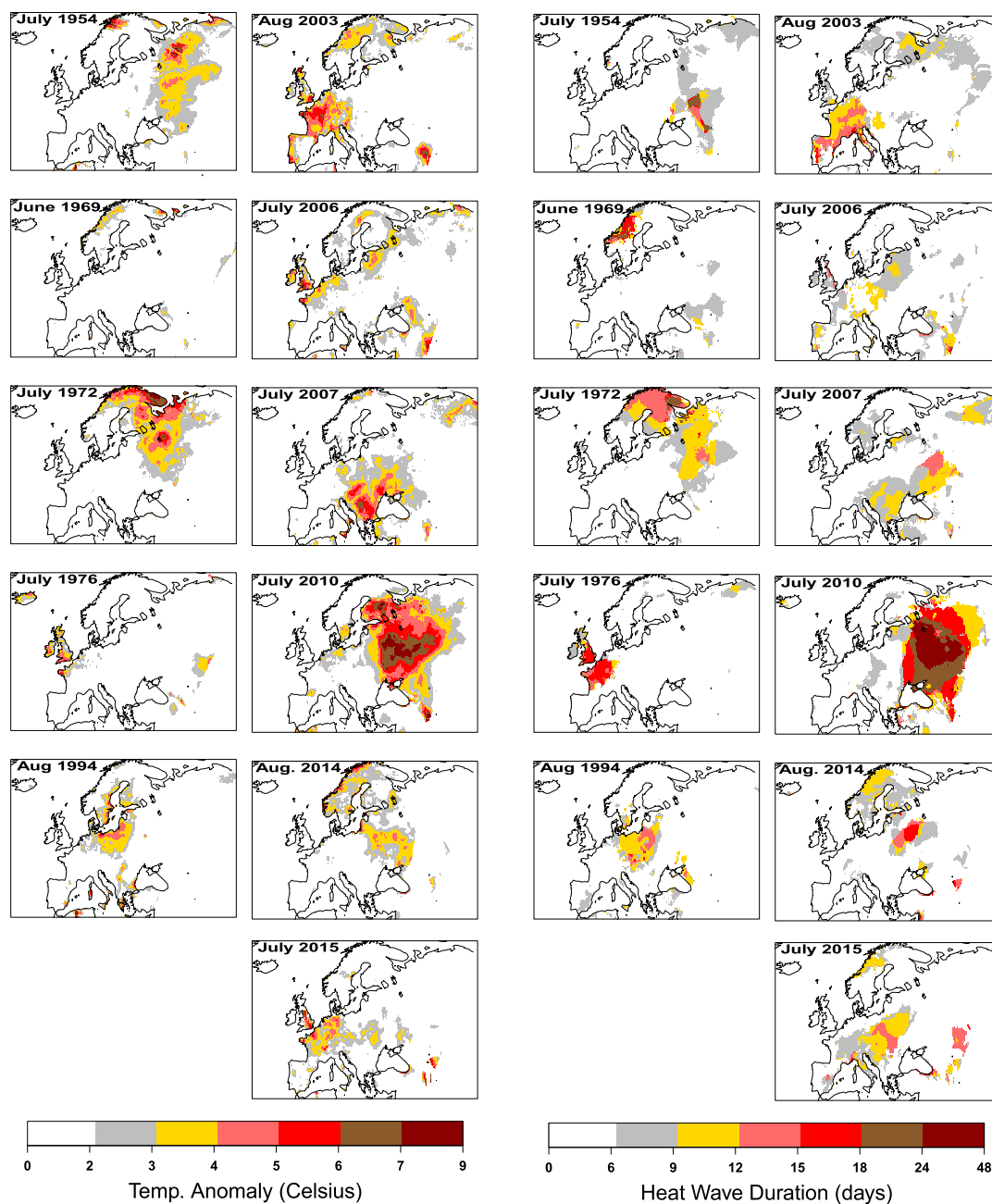
Figure A3. Temperature anomaly calculated following the definition in section 2.6 and heatwave duration of the top 10 European heatwaves and of the most recent heatwave of summer 2015.
